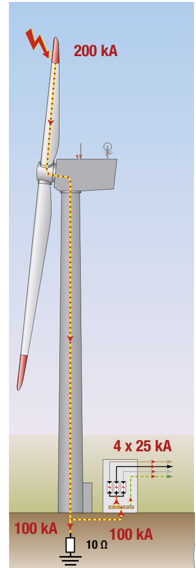
Fig. 4: Partitioning of the lightning current
