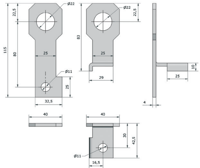
Dimension of IF1-22-W and IF3-22-F
